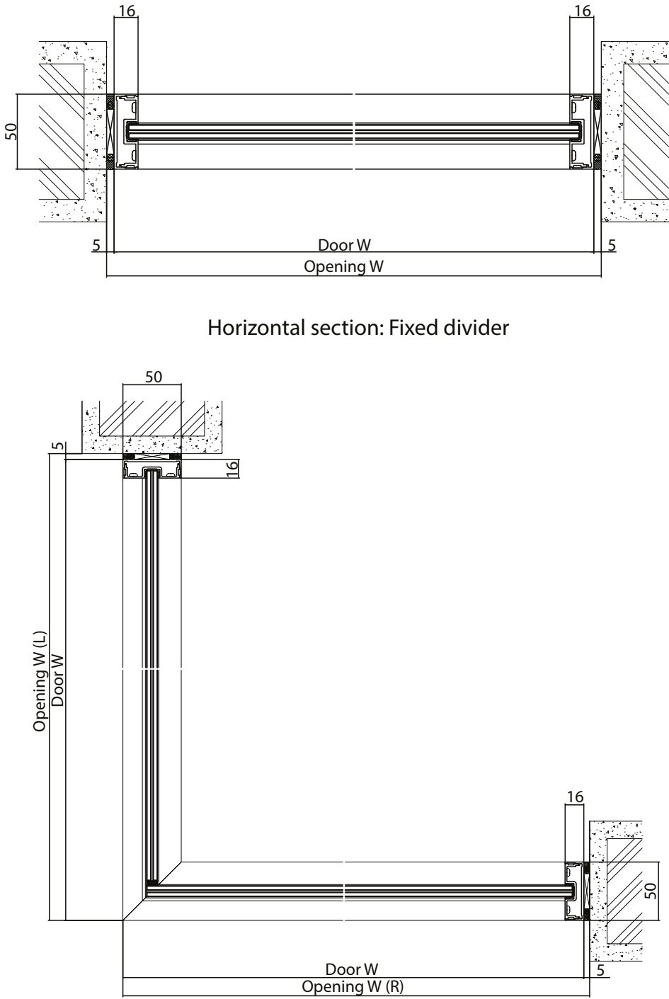
Horizontal section: Corner fixed divider
