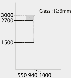
Pivot hinge without lock, divider handle, and divider lattice (H, H2)
