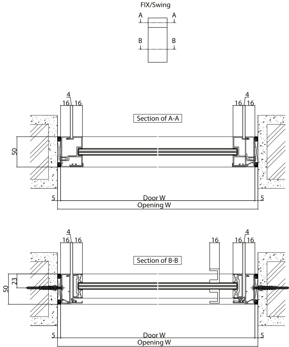
Horizontal section: Swing door R (Pivot hinge) with top FIX
